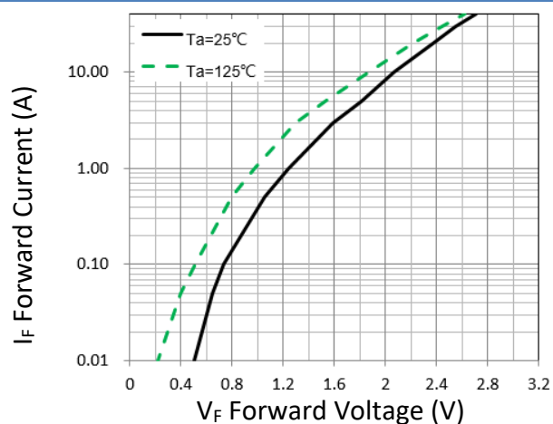
Figure 1. Forward Characteristic(typ.)
