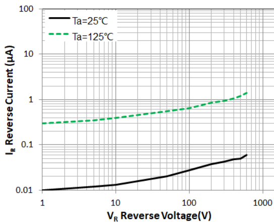
Figure 2. Reverse Characteristic(typ.)
