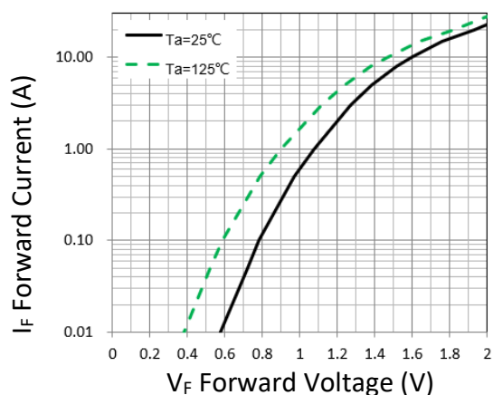
Figure 1. Forward Characteristic(typ.)
