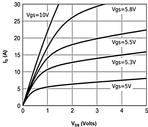
Figure 1: On-Region Characteristics
