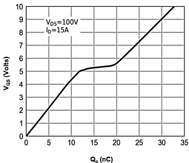
Figure 7: Gate-Charge Characteristics
