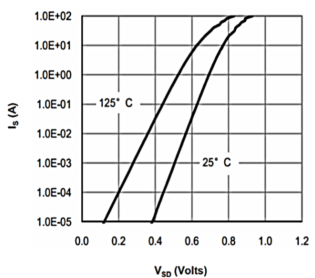
Figure 6: Body-Diode Characteristics
