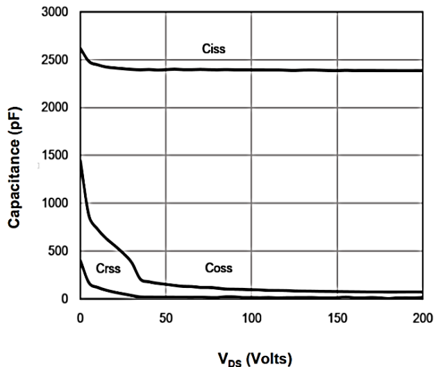
Figure 8: Capacitance Characteristics
