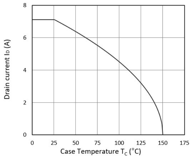
Figure 13. Drain Current vs. Temperature
