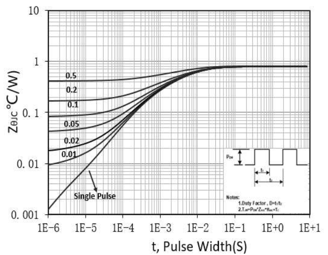
Figure 12. Transient Thermal Response Curve (TO-252)
