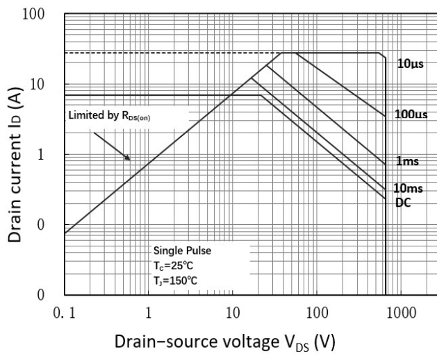
Figure 11. Maximum Safe Operating Area (TO-252)
