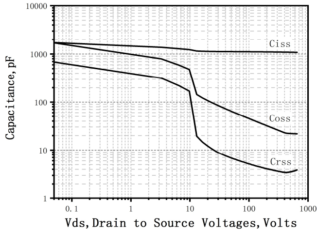
Figure 7. Capacitance Characteristics
