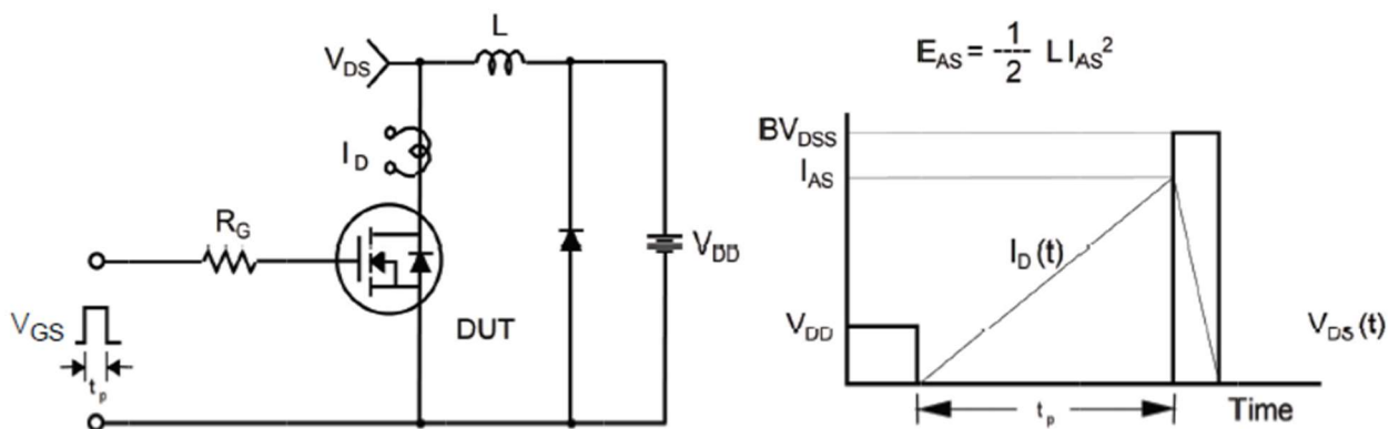
Unclamped Inductive Switching Test Circuit &amp; Waveforms
