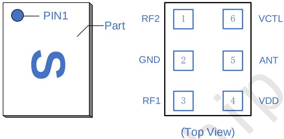
Figure 2 Pin-out Information
