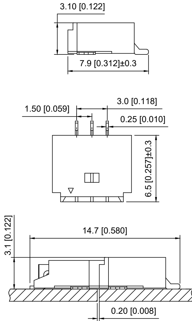
Assembly Layout
