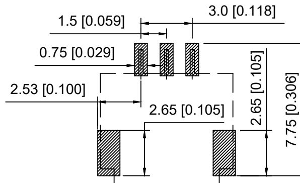
Board Layout General Tolerance:±0.05
