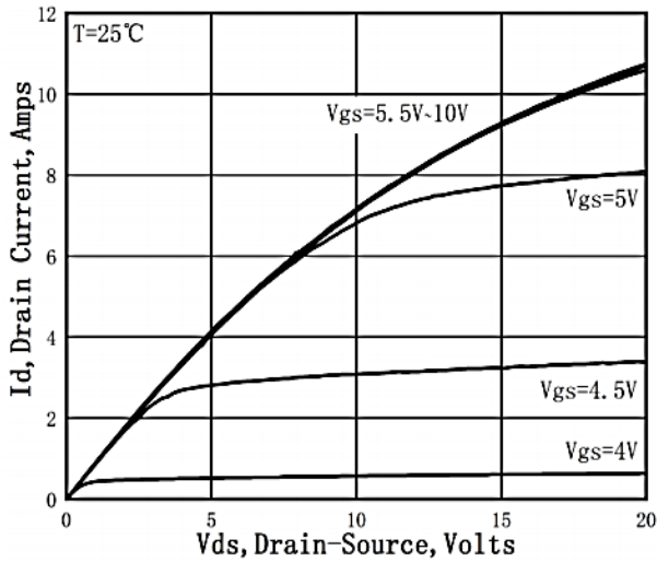
Figure 1. On-Region Characteristics
