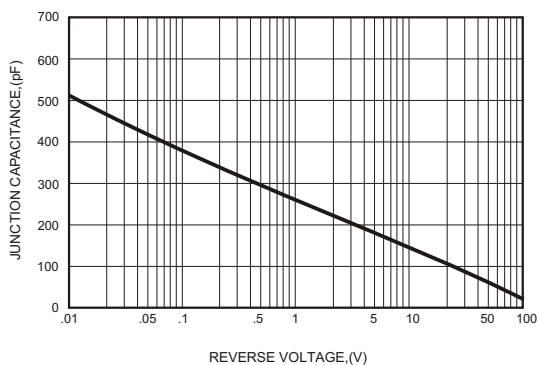
FIG.5-TYPICAL JUNCTION CAPACITANCE
