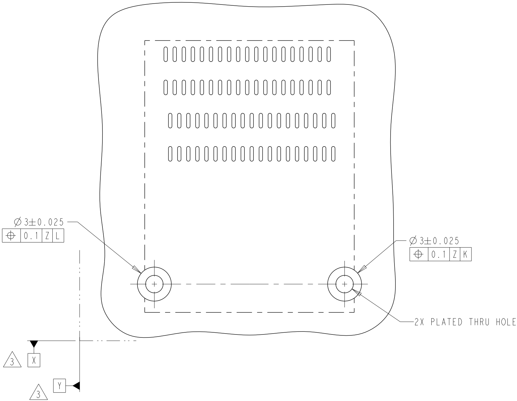
2474708-2/-3/-4/-5 RECOMMENDED PCB LAYOUT SAME AS 2474708-1 EXCEPT AS NOTED
