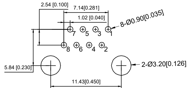
RECOMMENDED PCB LAYOUT VIEWED FROM COMPONENT SIDE
