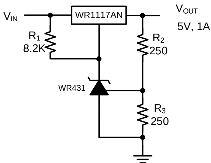
Precision 5V 1A Regulator
