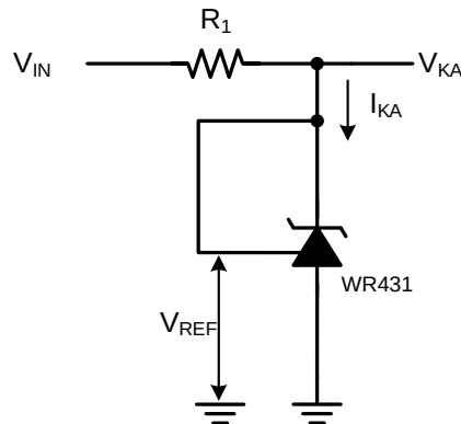
Test Circuit 1 for V_{KA} = V_{REF}
