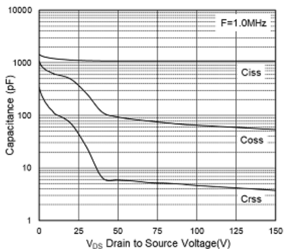
Fig.7 Capacitance
