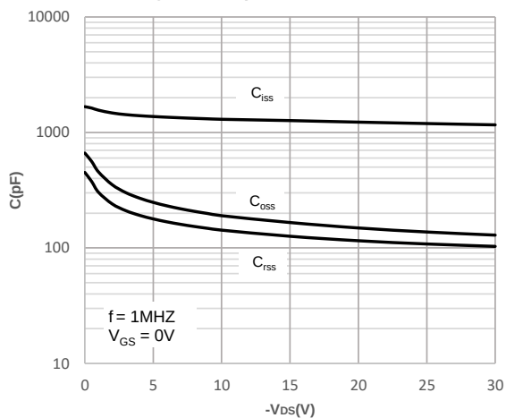
Figure 6: Capacitance Characteristics
