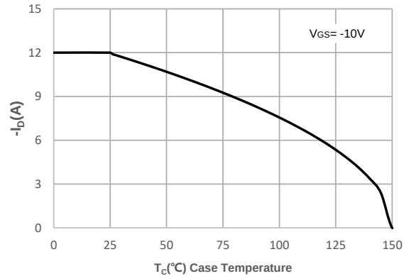
Figure 10: Maximum Continuous Driand Current vs. Case Temperature
