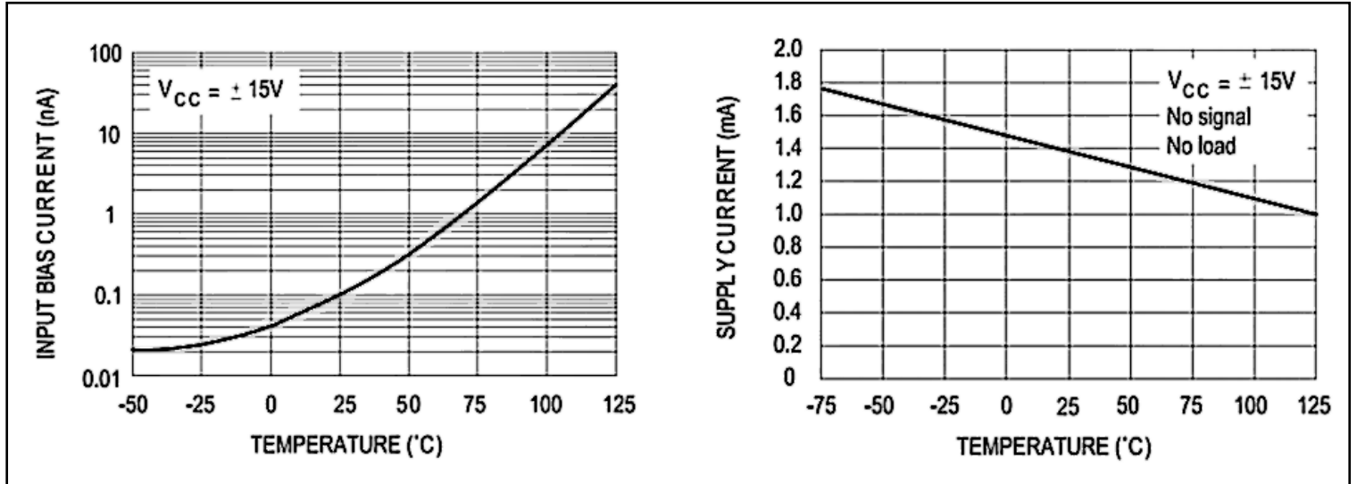
Figure 3 Relationship between input bias current and ambient temperature
