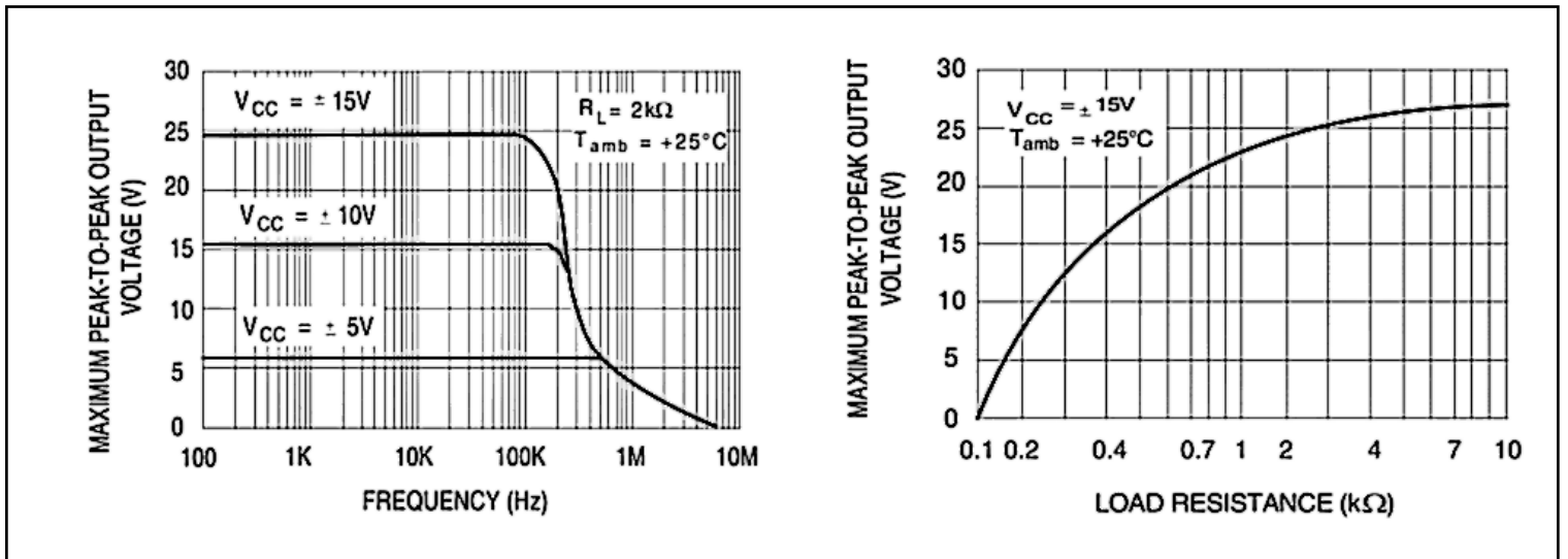
Figure 5 Relationship between maximum output voltage swing and frequency
