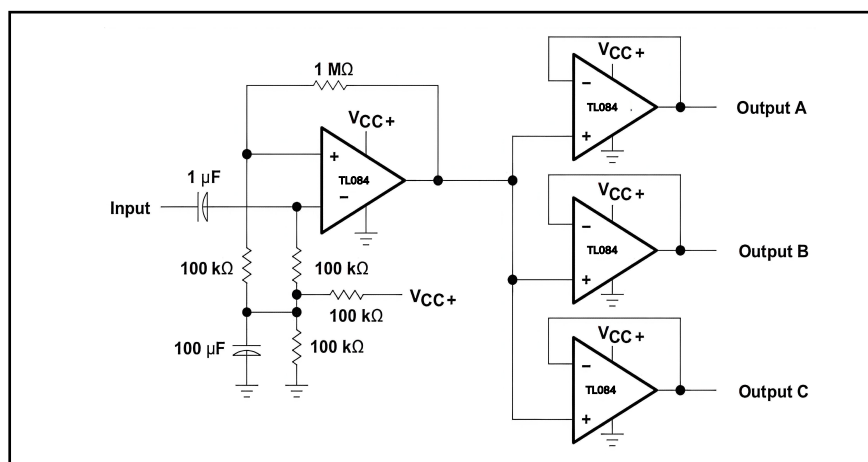
Figure 2 Audio distribution amplifier
