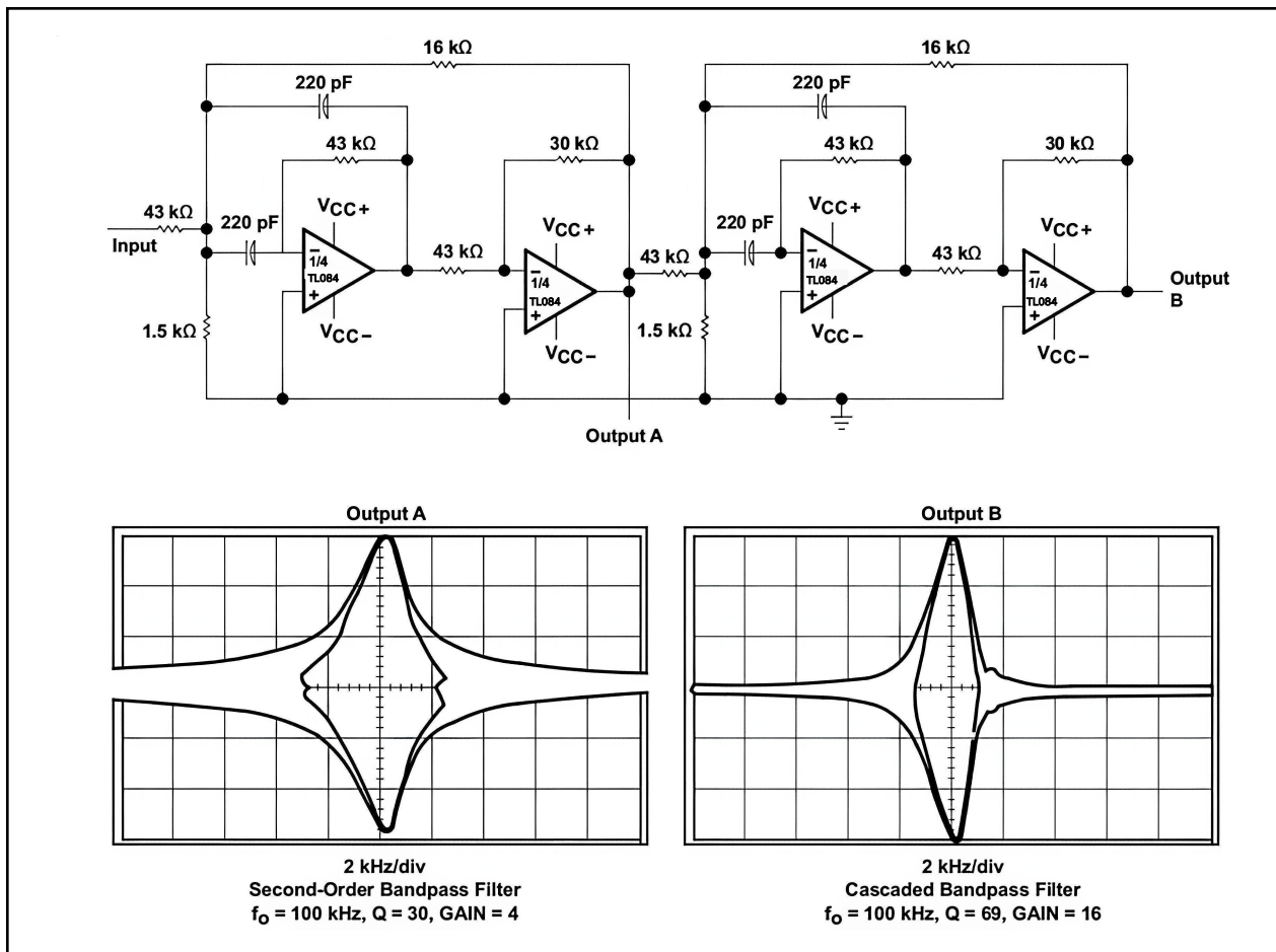
Figure 1 Positive feedback bandpass filter
