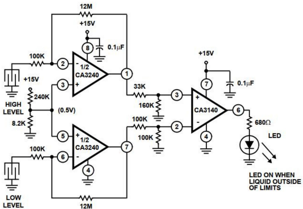
Figure 9: Dual-Level Detector
