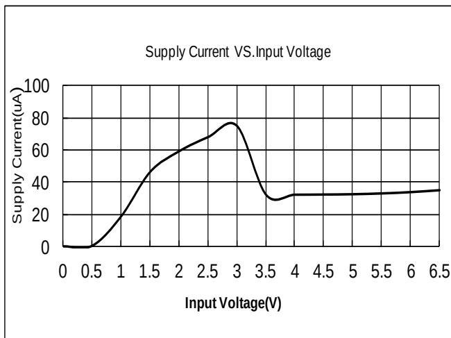
ME6211C18M5G
