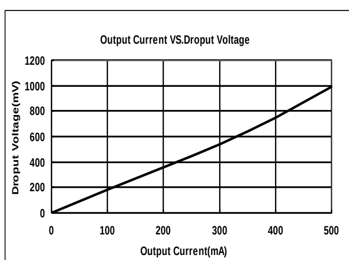
ME6211C18M5G
