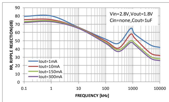
ME6211C18M5G
