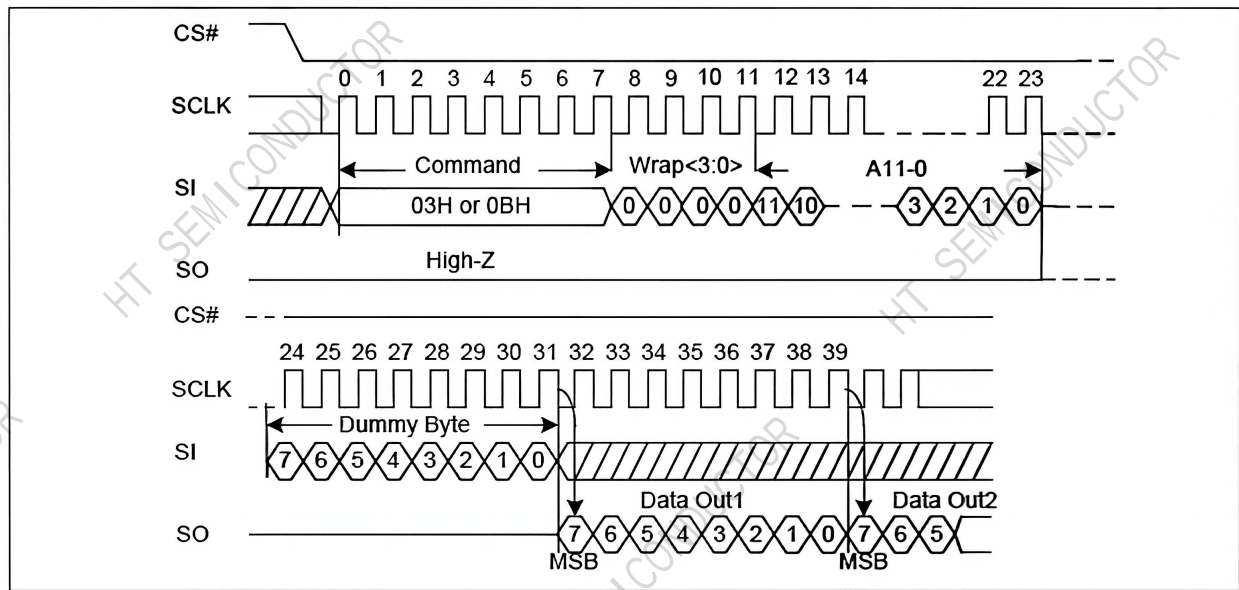
Figure 5-11 Read From Cache Sequence Diagram
