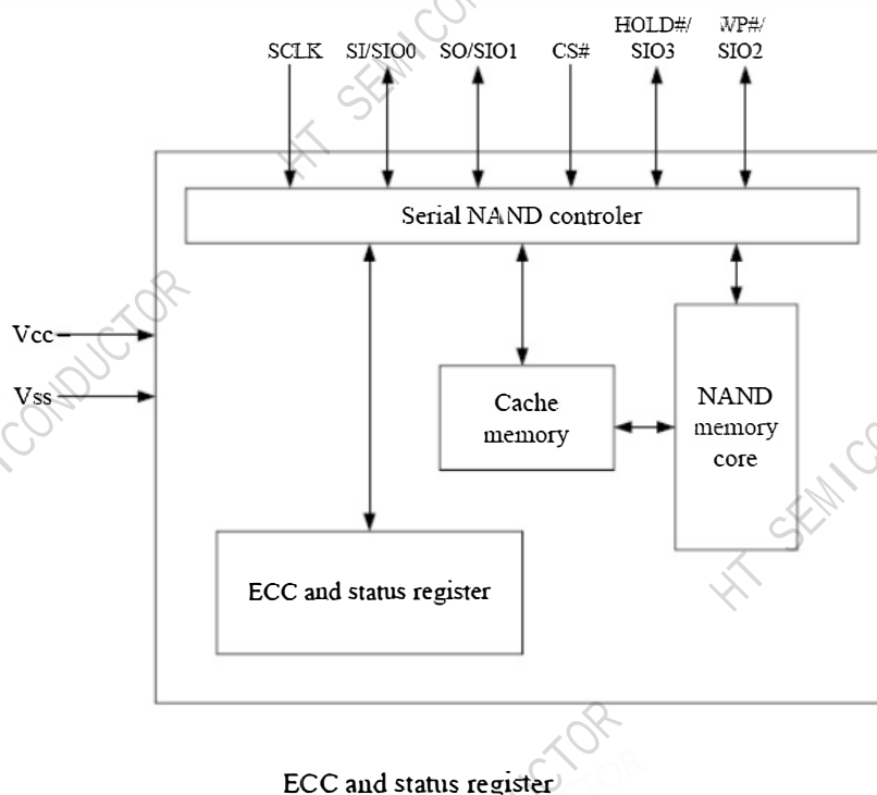
Figure 2-2 SPI NAND Flash Memory BLOCK DIAGRAM
