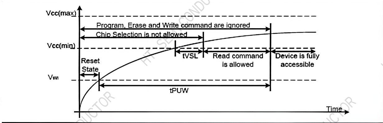
Figure 7-1 Power on Timing Sequence
