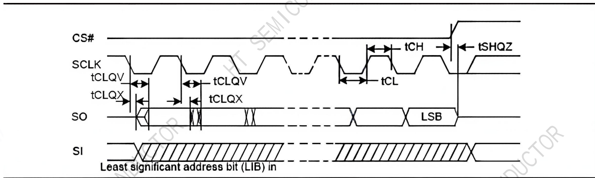
Figure 8-2 Output Timing
