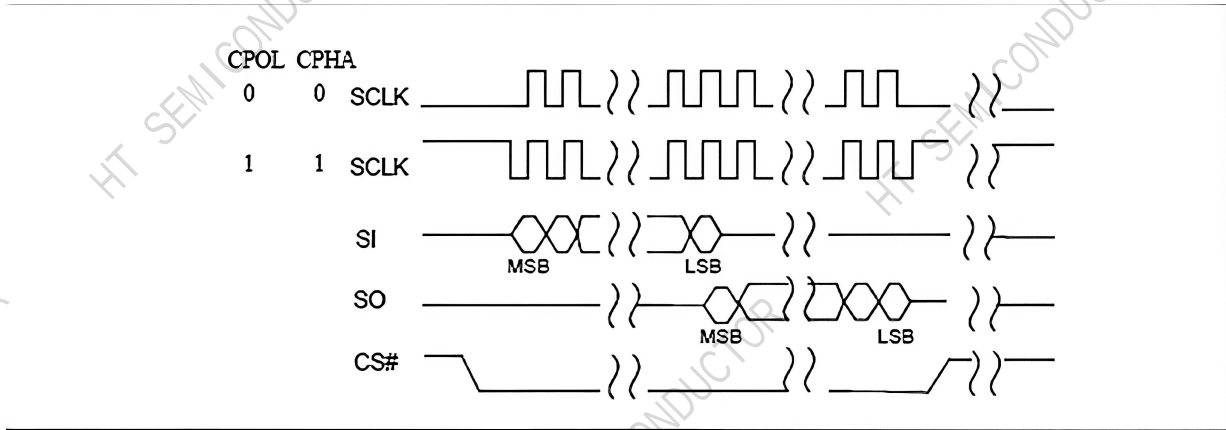
Figure 3-1 SPI Modes Sequence Diagram
