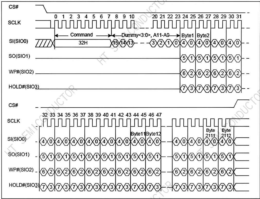
Figure 5-19 Program Load x4 Sequence Diagram
