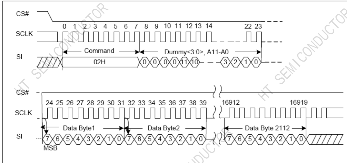
Figure 5-18 Program Load Sequence Diagram
