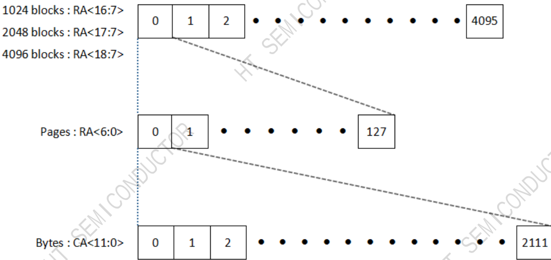
Figure 2-4 SPI NAND Flash(128 pages) MEMORY MAPPING
