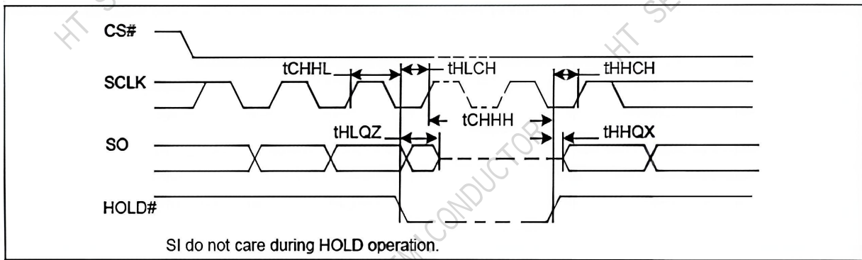
Figure 8-3 Hold Timing
