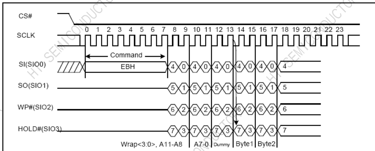
Figure 5-15 Read From Cache Quad IO Sequence Diagram
