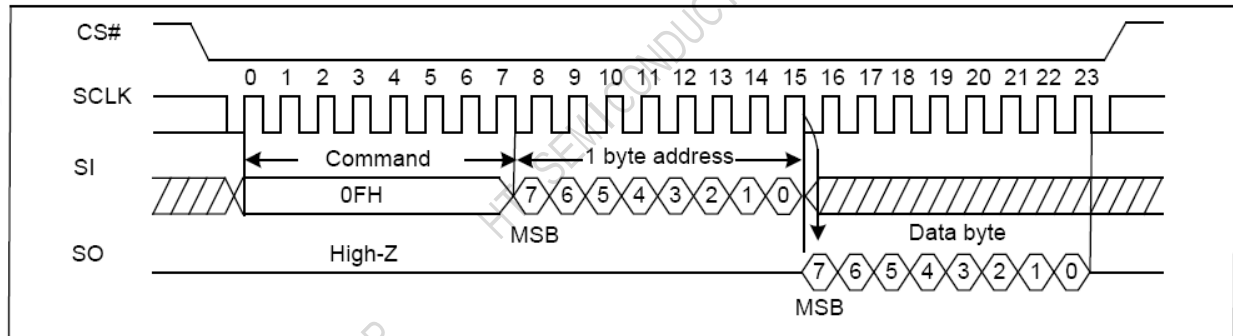
Figure 5-6 Get Features Sequence Diagram
