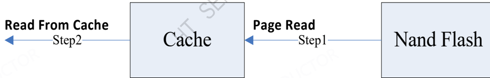
Figure 5-8 Page Read Operations Diagram
