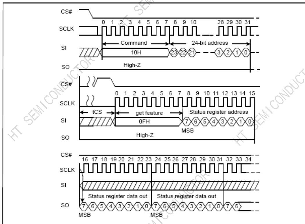
Figure 5-17 Program Execute Sequence Diagram
