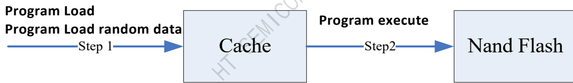
Figure 5-16 Page Program Operations Diagram
