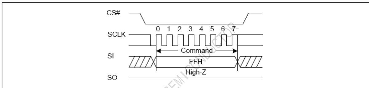
Figure 5-1 Reset Sequence Diagram
