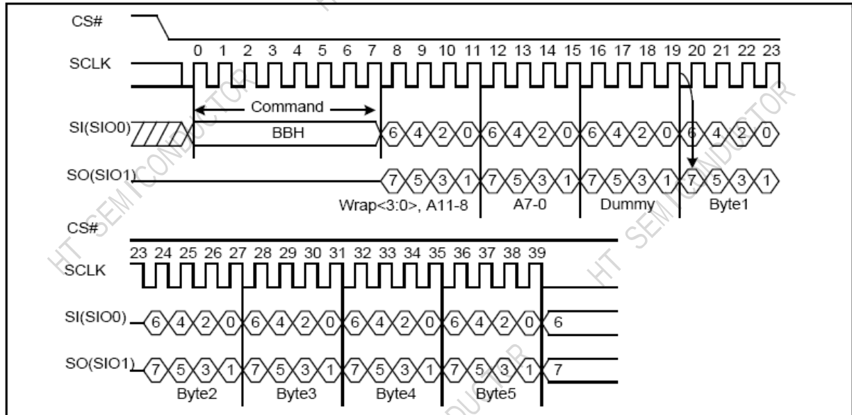
Figure 5-14 Read From Cache Dual IO Sequence Diagram
