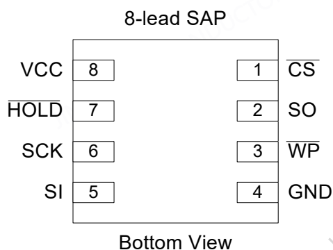
Figure 2-1. Connect Diagram
