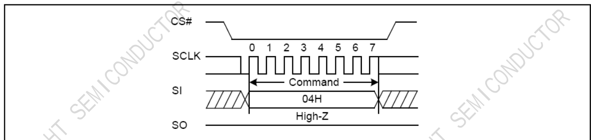
Figure 5-4 Write Disable Sequence Diagram
