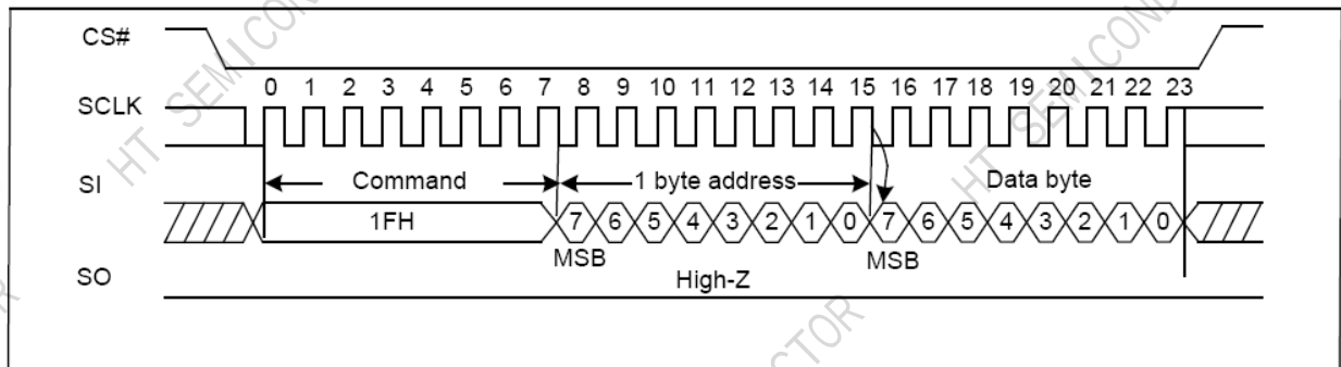
Figure 5-7 Set Features Sequence Diagram
