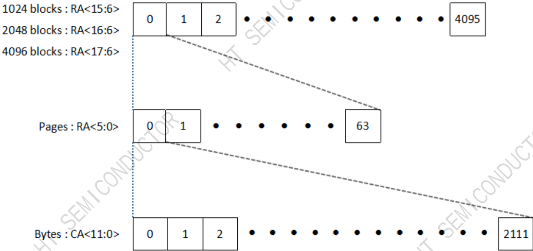
Figure 2-3 SPI NAND Flash(64 pages) MEMORY MAPPING
