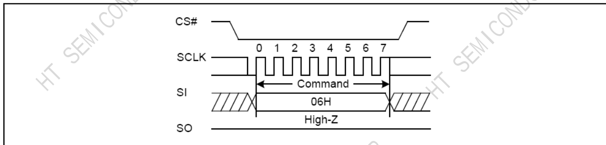
Figure 5-3 Write Enable Sequence Diagram
