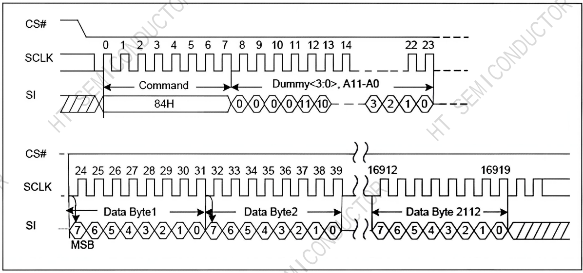
Figure 5-20 Program Load Random Data Sequence Diagram
