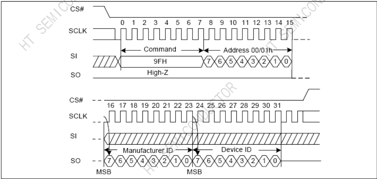
Figure 5-2 Read ID Sequence Diagram
