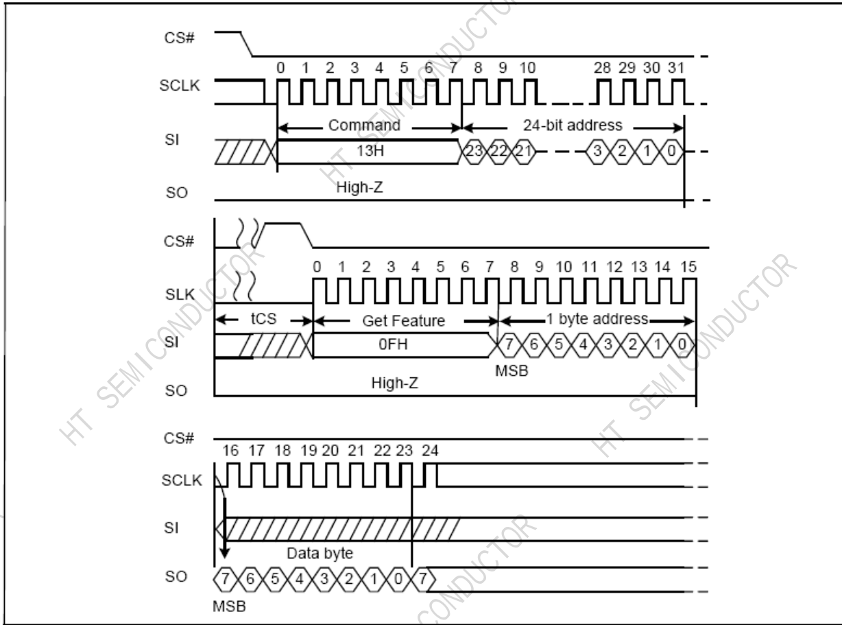
Figure 5-10 Page Read to cache Sequence Diagram
