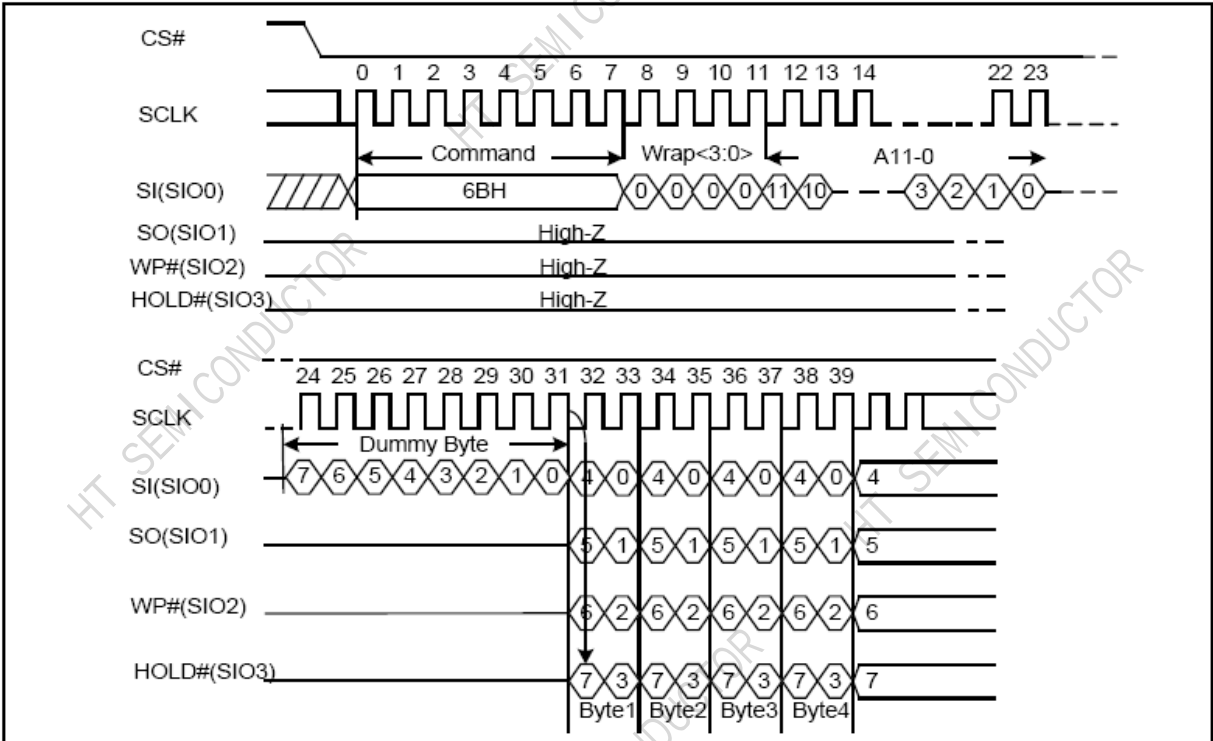
Figure 5-13 Read From Cache x4 Sequence Diagram
