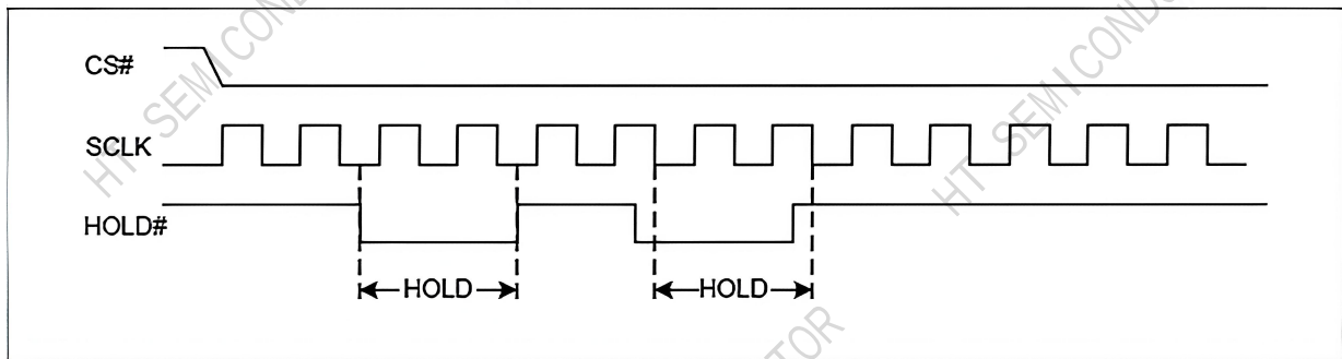
Figure 3-2 HOLD condition
