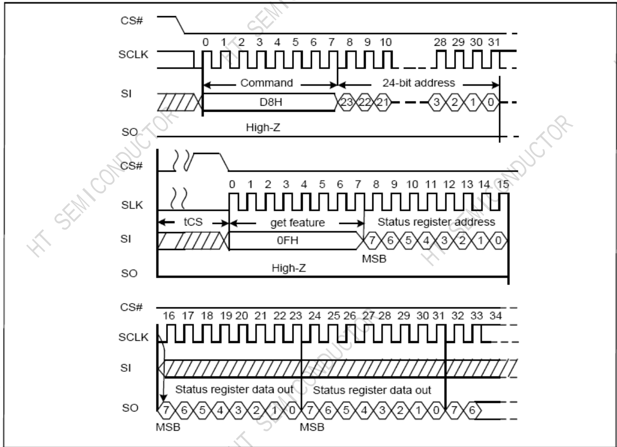
Figure 5-23 Block Erase Sequence Diagram
