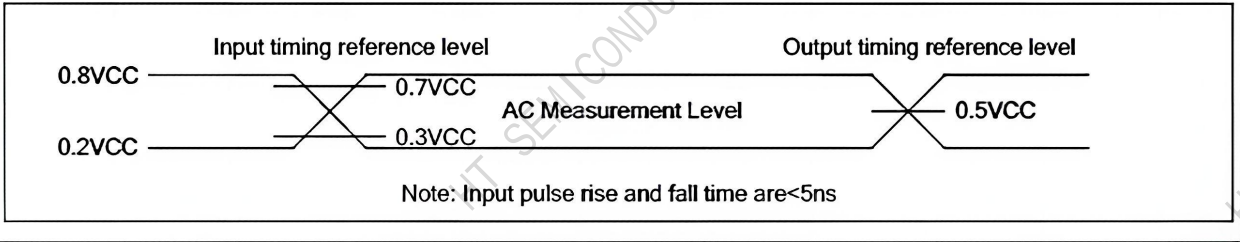
Figure 7-2 Input Test Waveform And Measurement Level
