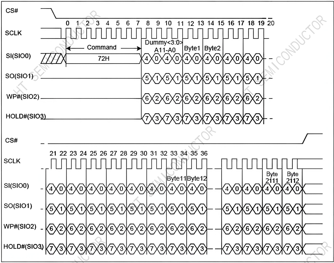
Figure 5-22 Program Load Random Data Quad IO Sequence Diagram
