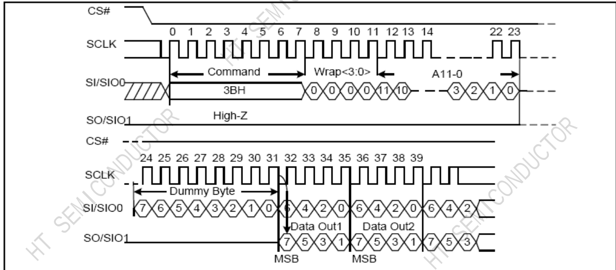
Figure 5-12 Read From Cache x2 Sequence Diagram
