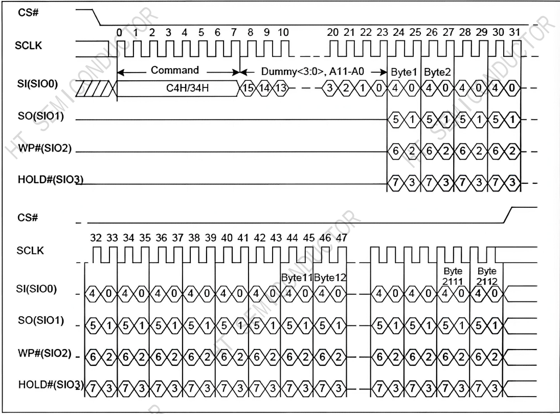
Figure 5-21 Program Load Random Data x4 Sequence Diagram
