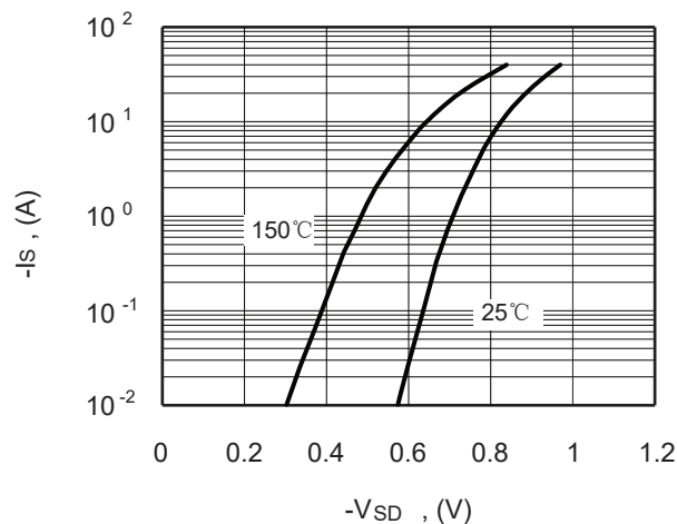
Body-Diode Characteristics
