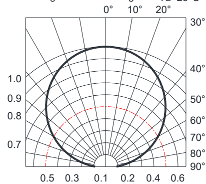
Fig.6-Radiation Diagram Ta=25°C
