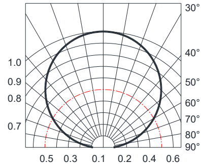
Fig.6-Radiation Diagram T_a=25^{\circ}\text{C}
