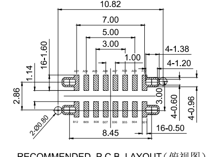
RECOMMENDED P.C.B. LAYOUT (俯视图) TOLERANCE UNSPECIFIED ±0.05mm
