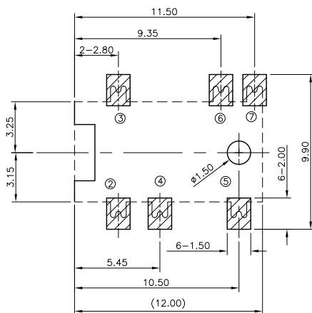
RIGHT PACKING P.C.B LAYOUT TOP VIEW
