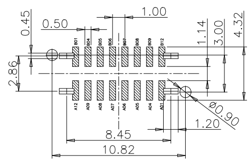
RECOMMENDED P. C. B. LAYOUT (俯视图) TOLERANCE UNSPECIFIED ±0.05mm
