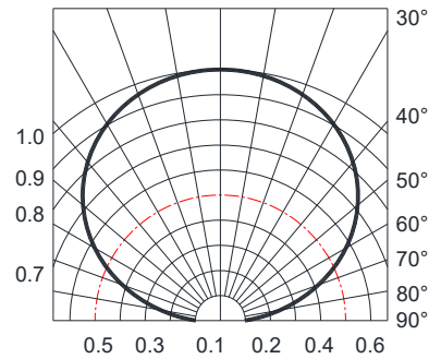
Fig.6-Radiation Diagram Ta=25°C
