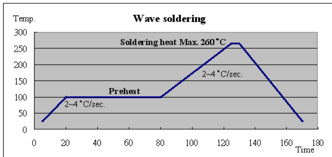
Lamp wave soldering profile :
