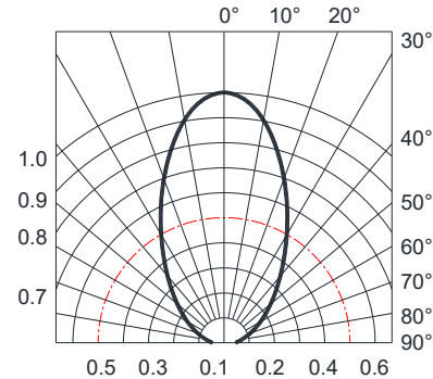
Fig.6-Radiation Diagram T_a=25^{\circ}\text{C}
