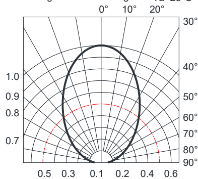
Fig.6-Radiation Diagram T_a=25^{\circ}\text{C}
