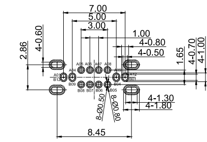
RECOMMENDED P.C.B. LAYOUT (俯视图) TOLERANCE UNSPECIFIED ±0.05mm
