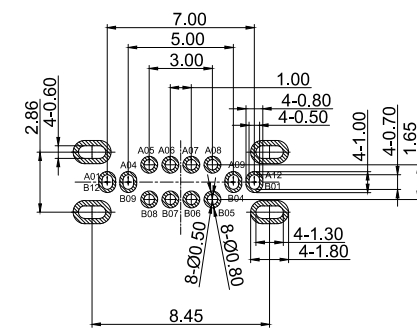
RECOMMENDED P.C.B. LAYOUT(俯视图) TOLERANCE UNSPECIFIED \pm 0.05 mm
