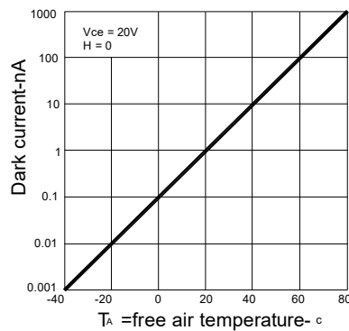
Fig.3 Dark current vs Free-air temperature
