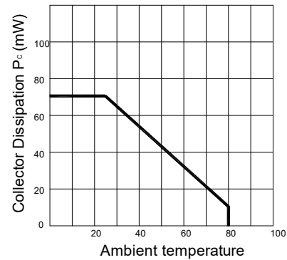
Fig.2 Ambient temperature vs. Collector Dissipation
