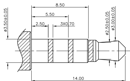
(Ø3.50mm 3 OR 4 POLE PLUG DETAIL DRAWING)
