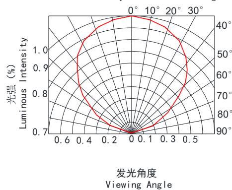
Fig. 6-光强与角度图(Ta=25°C) Luminous Intensity vs. Radiation Diagram
