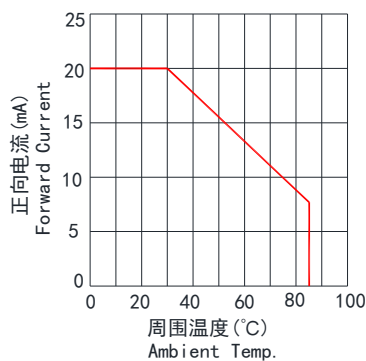
Fig. 5-正向电流与温度图 Forward Current vs. Ambient Temp.
