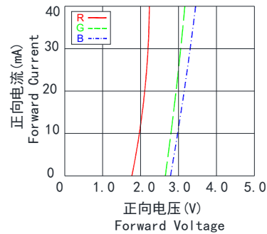
Fig. 2-正向电流与正向电压图(Ta=25°C) Forward Current vs. Forward Voltage
