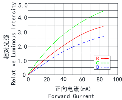
Fig. 4-相对光强与正向电流图(Ta=25°C) Relative Luminous Intensity vs. Forward Current
