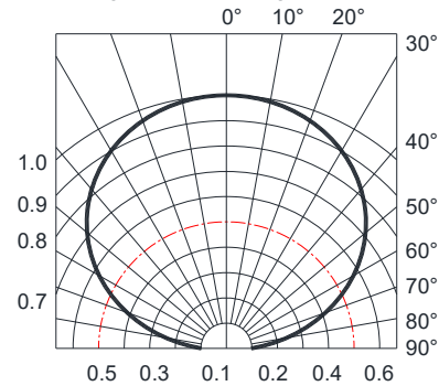
Fig.6-Radiation Diagram Ta=25℃
