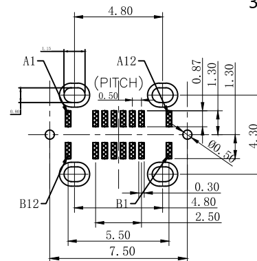
RECOMMENDED P.C.B. LAYOUT TOLERANCE UNSPECIFIED \pm 0.05\text{mm}
