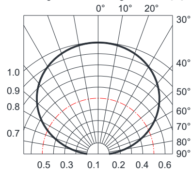
Fig.6-Radiation Diagram Ta=25°C
