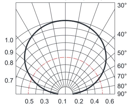
Fig.6-Radiation Diagram Ta=25°C
