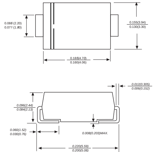
DO-214AA/SMB
