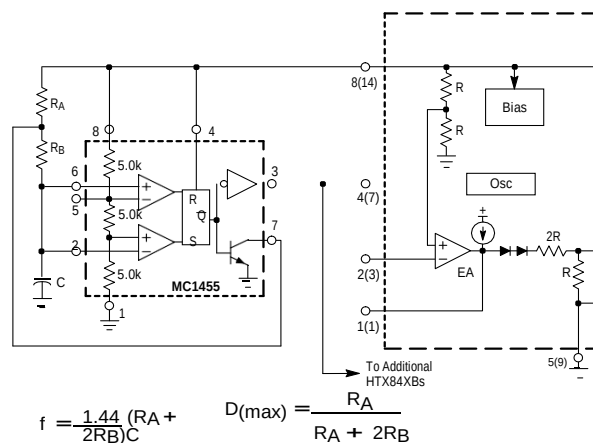
Figure 19. External Duty Cycle Clamp and Multi-Unit Synchronization
