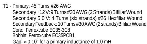
Figure 30. 7 W Off-Line Flyback Regulator
