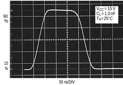
Figure 13. Output Waveform
