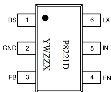
XTP8221D SOT23-6
