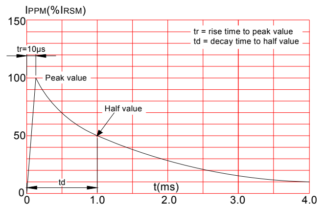
FIG.2: Pulse waveform
