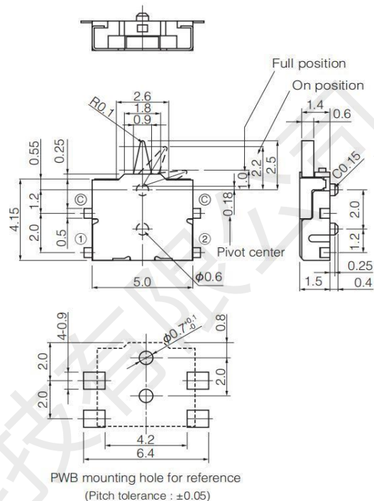
No. 2 ESE23F101 Straight terminal with boss (Without Boss ESE23F001)
