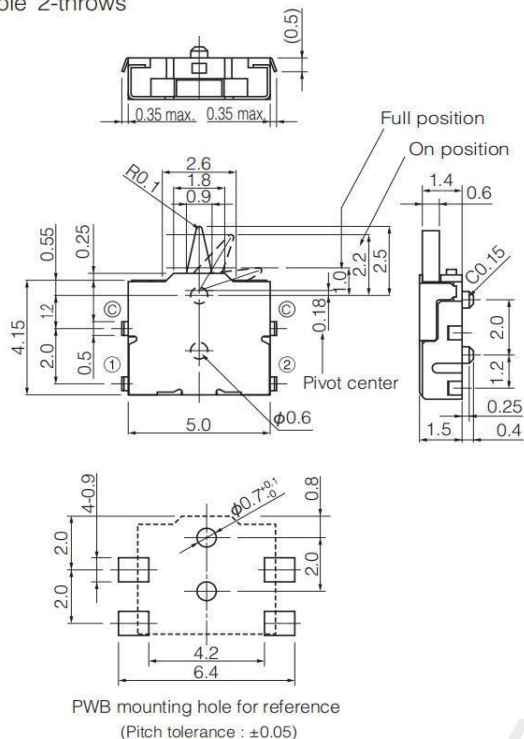
No. 1 ESE23J101 J-bent terminal with boss (Without Boss ESE23J001)
