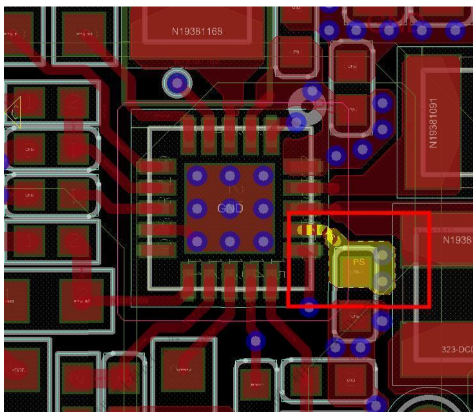
Figure 8-1 PCB reference
