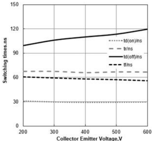
Figure 15. Typical Switching Times vs VCE ( T_J=25^{\circ}\text{C} , V_{GE}=15/0\text{V} , I_C=75\text{A} )
