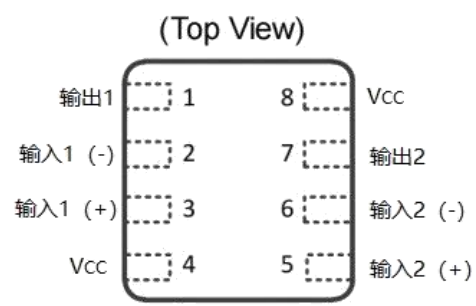
DFN-8 3*3
