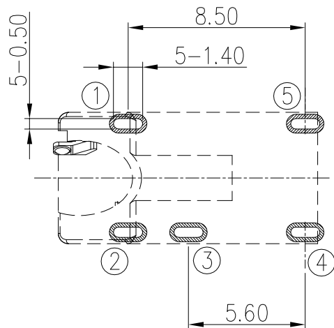
RECOMMENDED PCB LAYOUT (TOP VIEW) GENERAL TOLERANCES: \pm 0.05
