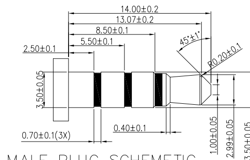
MALE PLUG SCHEMATIC
