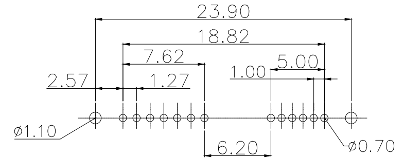
PCB LAYOUT
