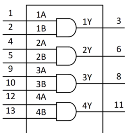
Fig. 1. Logic symbol
