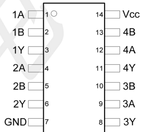
SOP-14
