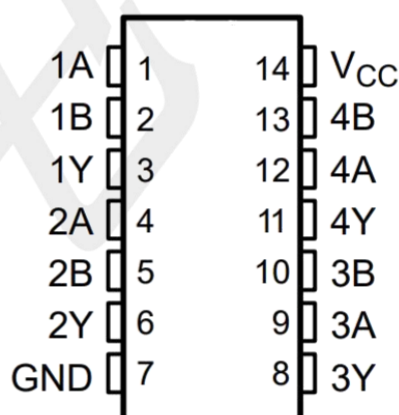
SOP-14
