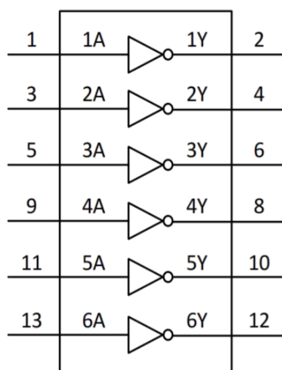
Fig. 1. Logic symbol
