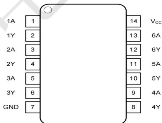
TSSOP-14
