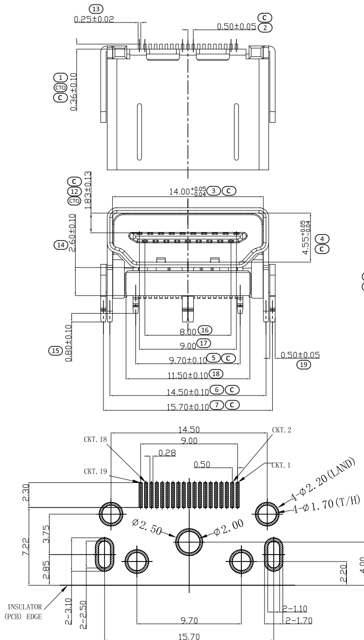
PCB PATTERN LAYOUT (T1.2±0.15)
