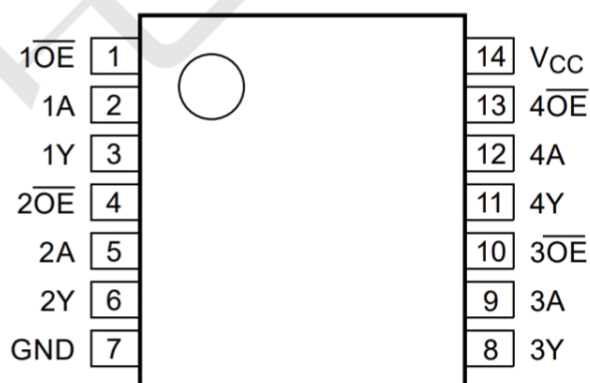
TSSOP-14
